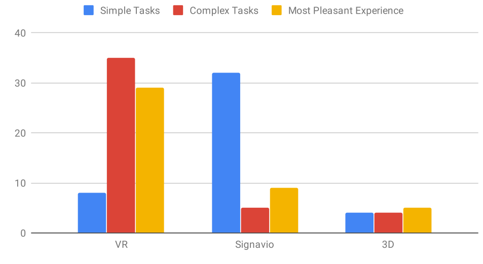
Participants preference after taking part in the experiment
